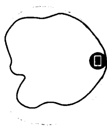
Figure 3: BeamFlex Antenna Pattern (5GHz)
